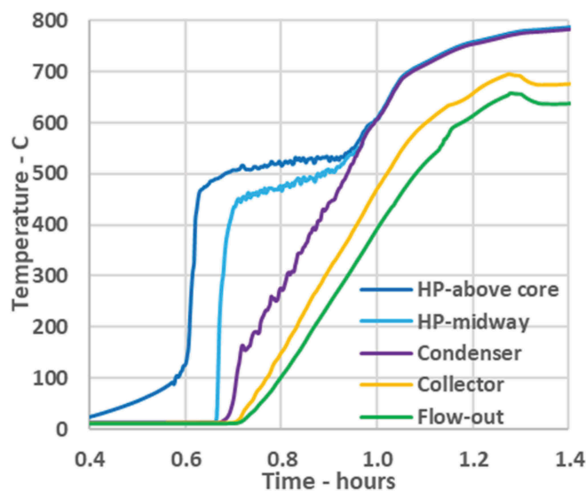
Fig. 8. Average temperatures of all six simulators.
