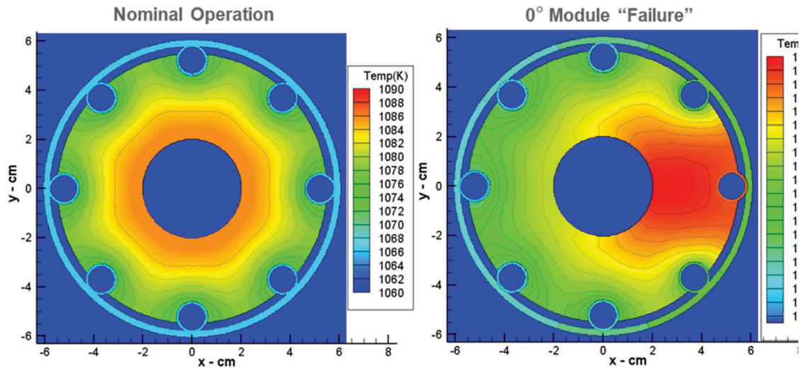
Fig. 17. Pretest models of the fuel temperature profile.
