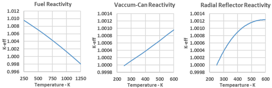
Fig. 14. Reactivity versus temperature for the fuel, vacuum can, and radial reflector.
