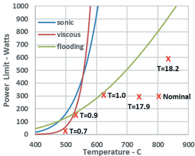
X marks KRUSTY heat pipe conditions at the denoted time
